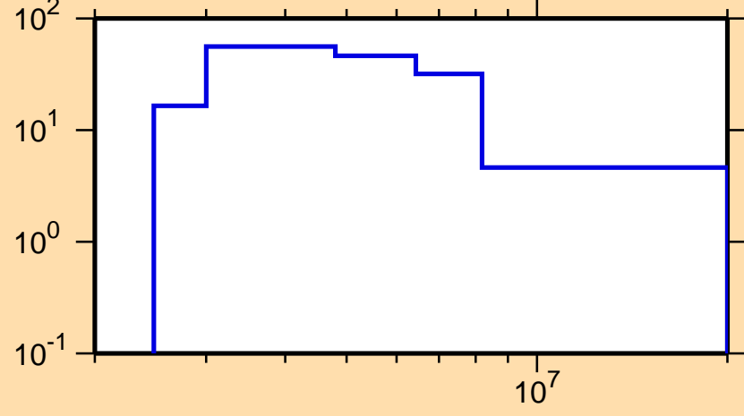
\Delta\sigma/\sigma vs. E for ^{277}
