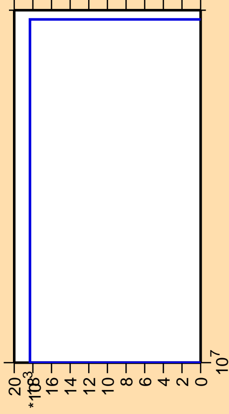
\Delta\sigma/\sigma vs. E for ^{279}
