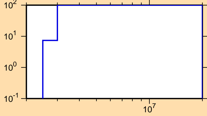
\Delta\sigma/\sigma vs. E for ^{279}
