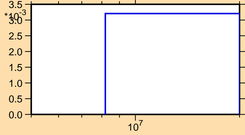
\sigma vs. E for ^{16}\text{N}(n,nd)
