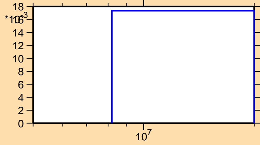
\sigma vs. E for ^{16}\text{N}(n,d)
