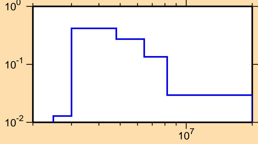
\sigma vs. E for ^{16}\text{N}(n,n_2)
