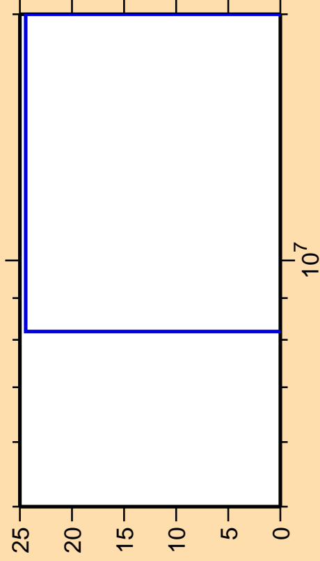
\Delta\sigma/\sigma vs. E for ^{16}\text{N}(\text{mt 11})
