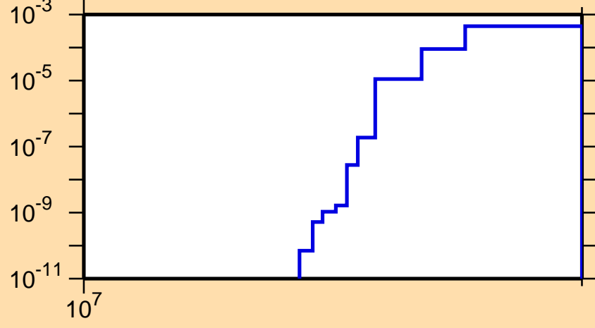
\sigma vs. E for ^{21}\text{Na}(n,pd)
