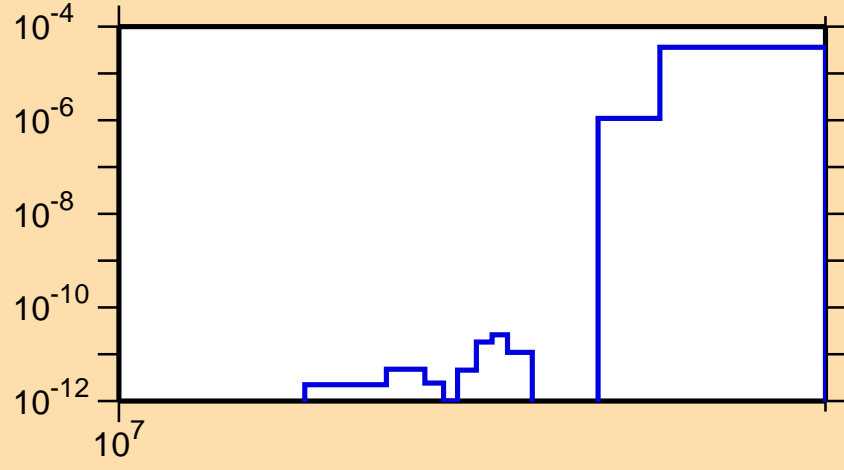
\sigma vs. E for ^{21}\text{Na}(n,t)
