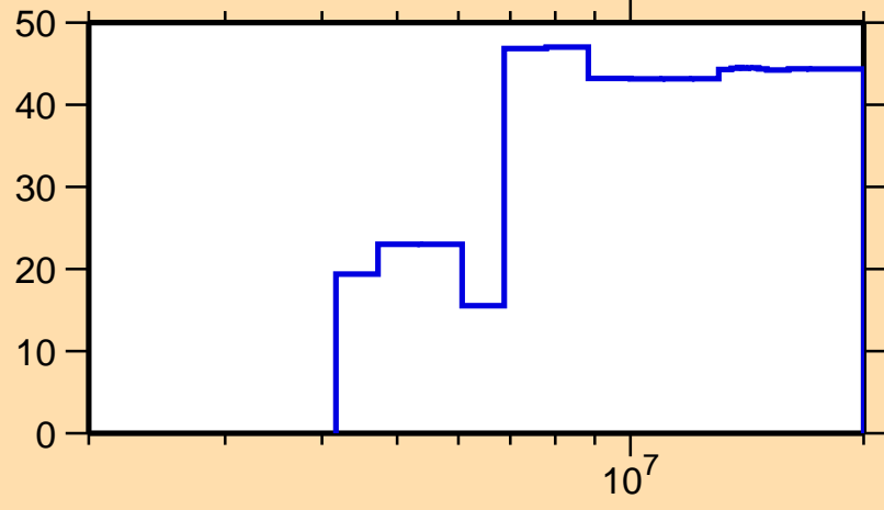
\Delta\sigma/\sigma vs. E for ^{21}\text{Na}(n,incl.)
