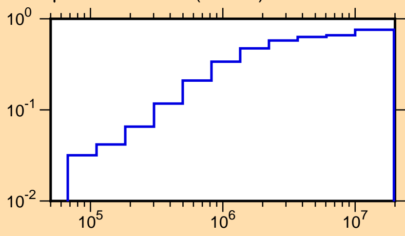
\mu vs. E for ^{21}\text{Na}(\text{mt251})
