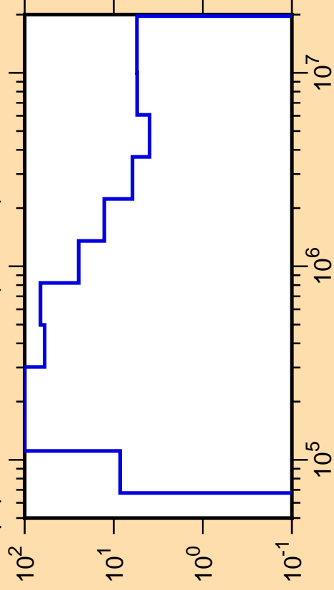
\Delta\mu/\mu vs. E for ^{21}\text{Na}(\text{mt251})
