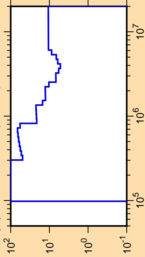
\Delta\mu/\mu vs. E for ^{22}\text{Na}(\text{mt251})
