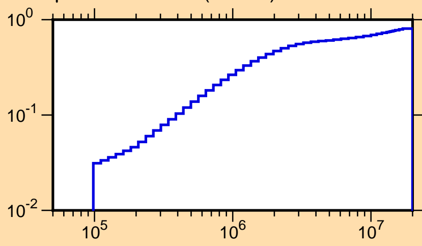
\mu vs. E for ^{22}\text{Na}(\text{mt251})
