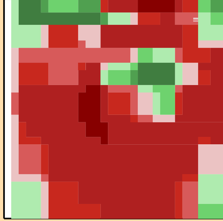
\Delta\sigma/\sigma vs. E for ^{22}\text{Na}(n,\text{inel.})
