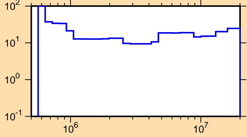
\Delta\sigma/\sigma vs. E for ^{22}\text{Na}(n,\text{inel.})
