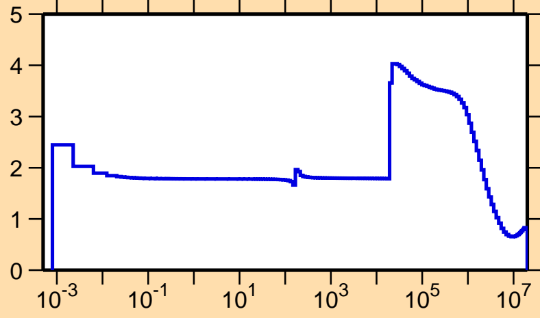
\sigma vs. E for ^{22}\text{Na}(n,\text{el.})
