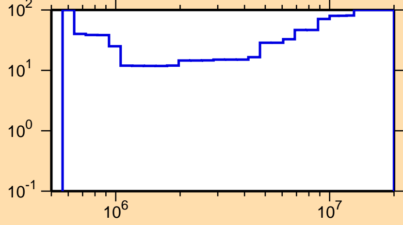
\Delta\sigma/\sigma vs. E for ^{22}\text{Na}(n,n_1)
