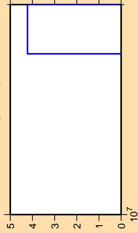
\Delta\sigma/\sigma vs. E for ^{22}\text{Na}(n,2n\alpha)
