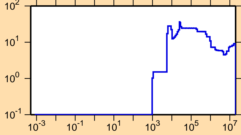
\Delta\sigma/\sigma vs. E for ^{22}\text{Na}(n,\text{nonel.})
