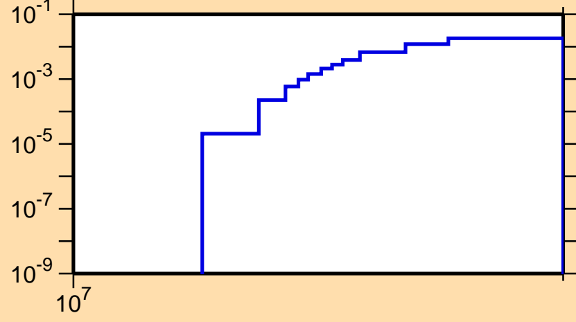
\sigma vs. E for ^{22}\text{Na}(n,\text{nd})
