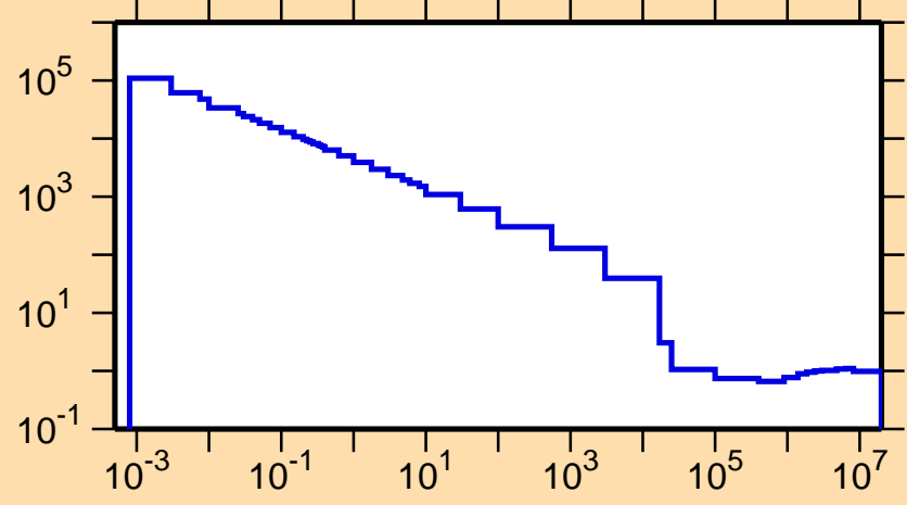
\sigma vs. E for ^{22}\text{Na}(n,\text{nonel.})
