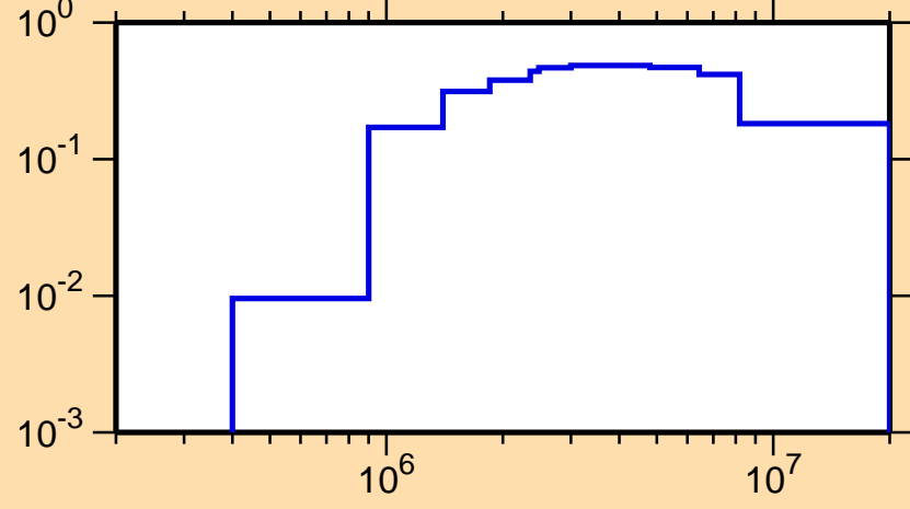
\sigma vs. E for ^{22}\text{Na}(n,\text{inel.})
