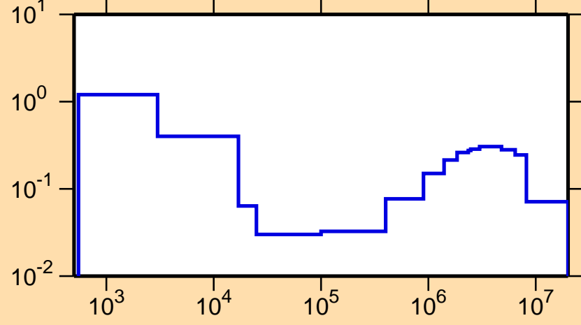
\sigma vs. E for ^{22}\text{Na}(n,\alpha)
