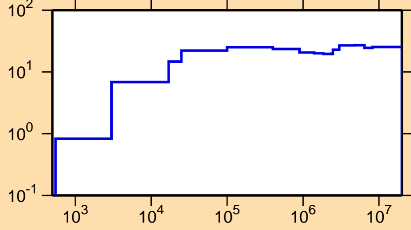
\Delta\sigma/\sigma vs. E for ^{22}\text{Na}(n,p)
