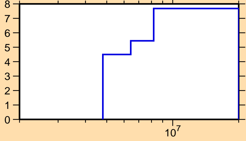
\Delta\sigma/\sigma vs. E for ^{22}\text{Na}(n,\text{nonel.})
