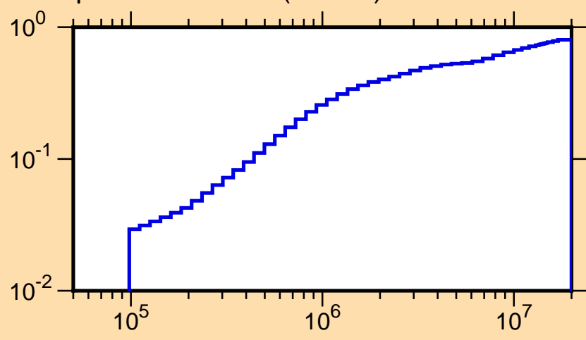
\mu vs. E for ^{23}\text{Na}(\text{mt251})
