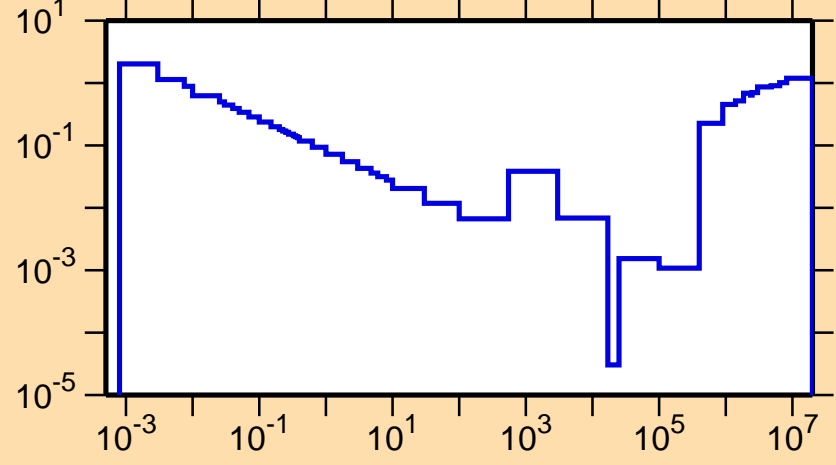
\sigma vs. E for ^{23}\text{Na}(n,\text{nonel.})
