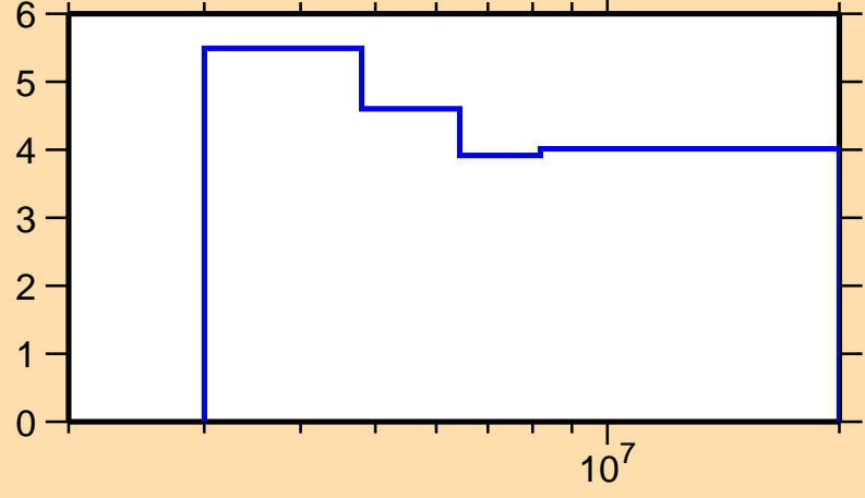
\Delta\sigma/\sigma vs. E for ^{23}\text{Na}(n,\text{nonel.})
