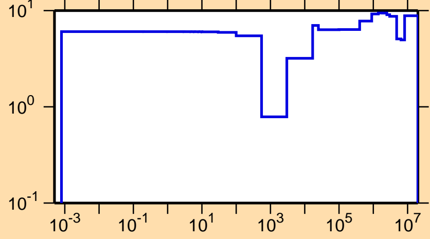
\Delta\sigma/\sigma vs. E for ^{23}\text{Na}(n,\text{el.})
