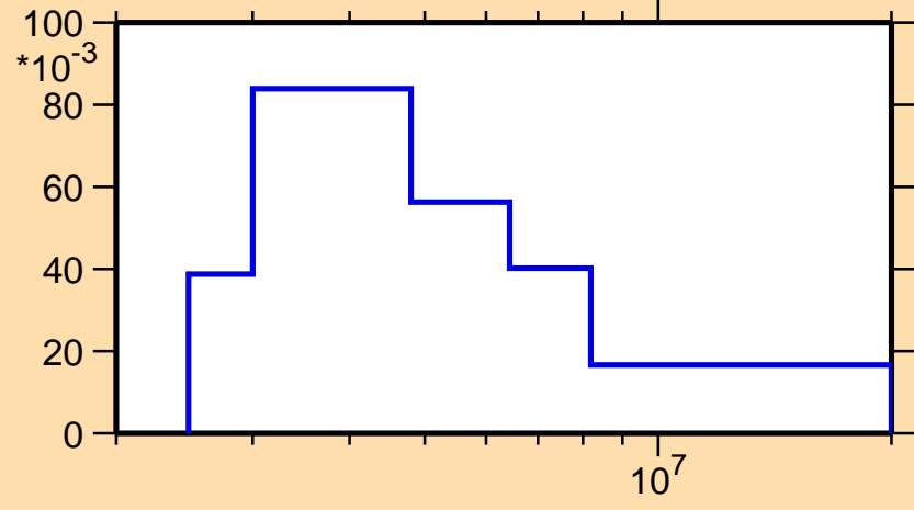
\sigma vs. E for ^{23}\text{Na}(n,n_3)
