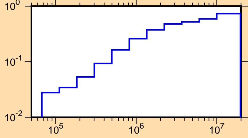
\mu vs. E for ^{24}\text{Na}(\text{mt251})
