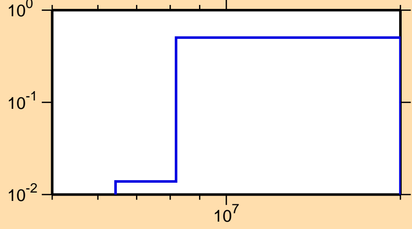
\sigma vs. E for ^{24}\text{Na}(n,2n)
