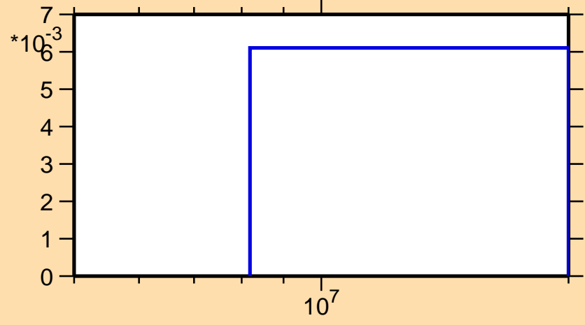
\sigma vs. E for ^{24}\text{Na}(n,np)
