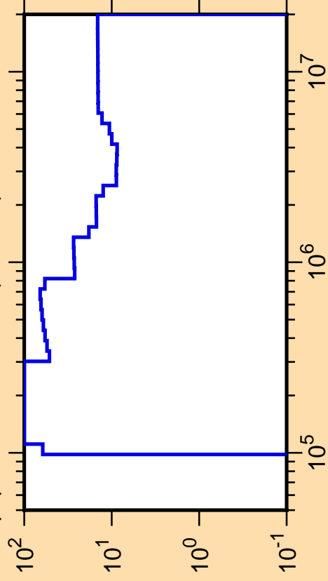
\Delta\mu/\mu vs. E for ^{25}\text{Na}(\text{mt251})
