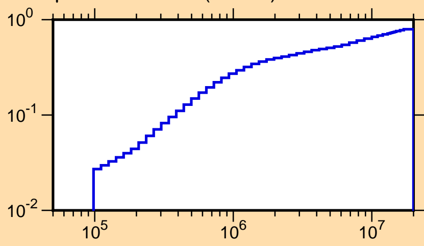
\mu vs. E for ^{25}\text{Na}(\text{mt251})
