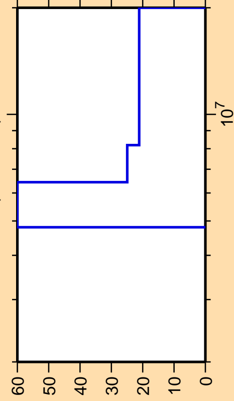
\Delta\sigma/\sigma vs. E for ^{25}\text{Na}(n,ncont.)
