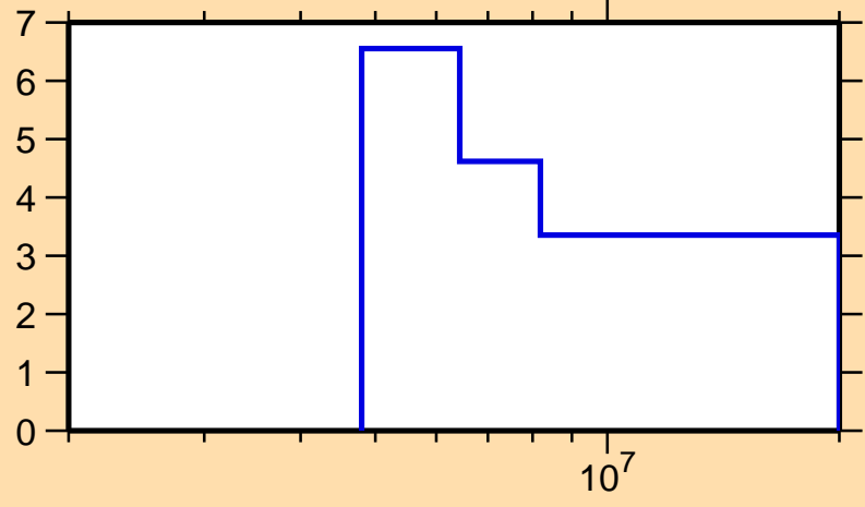
\Delta\sigma/\sigma vs. E for ^{25}\text{Na}(n,tot.)
