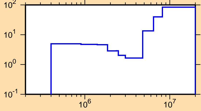
\Delta\sigma/\sigma vs. E for ^{26}\text{Na}(n,n_1)
