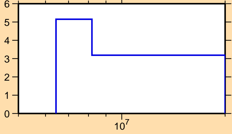
\Delta\sigma/\sigma vs. E for ^{26}\text{Na}(n,el.)
