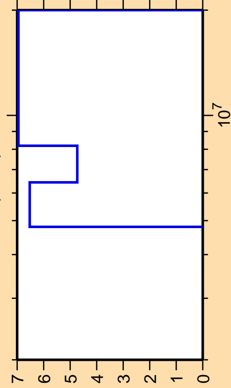
\Delta\sigma/\sigma vs. E for ^{26}\text{Na}(n,2n)
