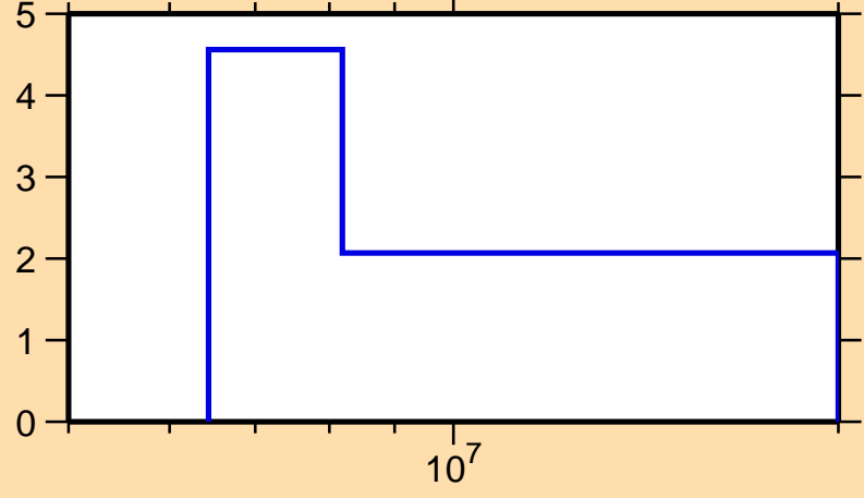
\Delta\sigma/\sigma vs. E for ^{26}\text{Na}(n,\text{tot.})
