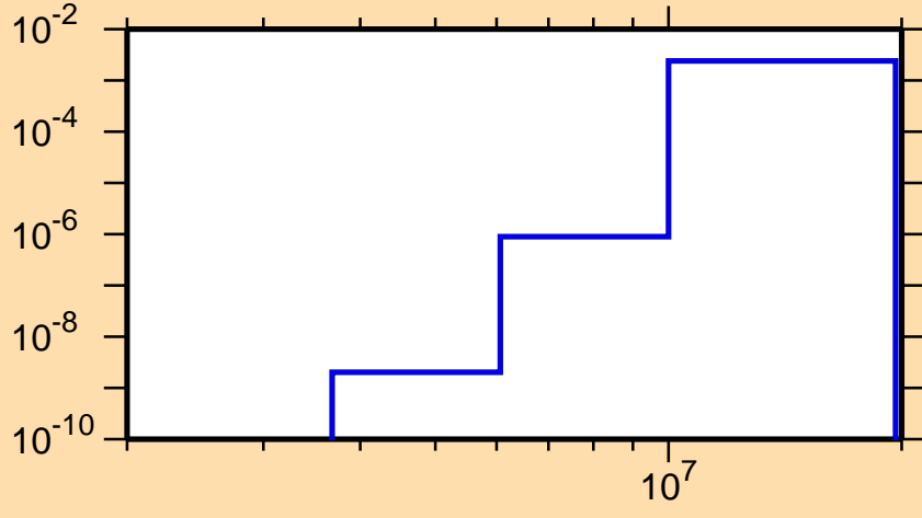
\sigma vs. E for ^{83}\text{Nb}(n,\text{He}3)
