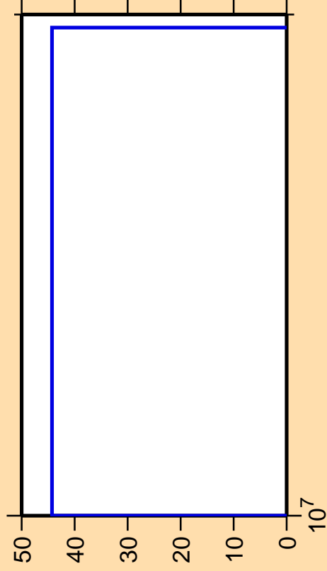
\Delta\sigma/\sigma vs. E for ^{83}\text{Nb}(n,ncont.)
