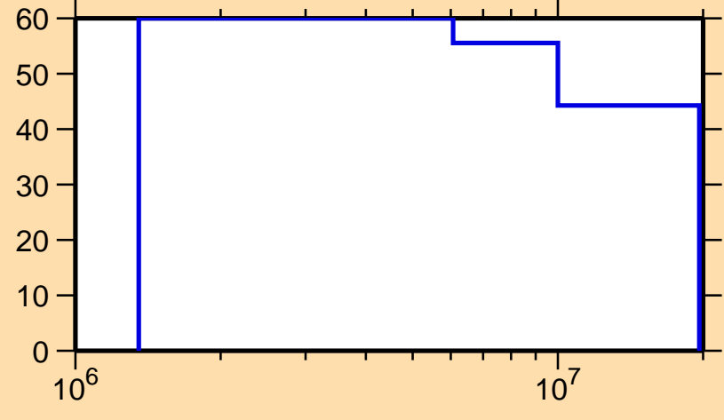
\Delta\sigma/\sigma vs. E for ^{83}\text{Nb}(n,ncont.)
