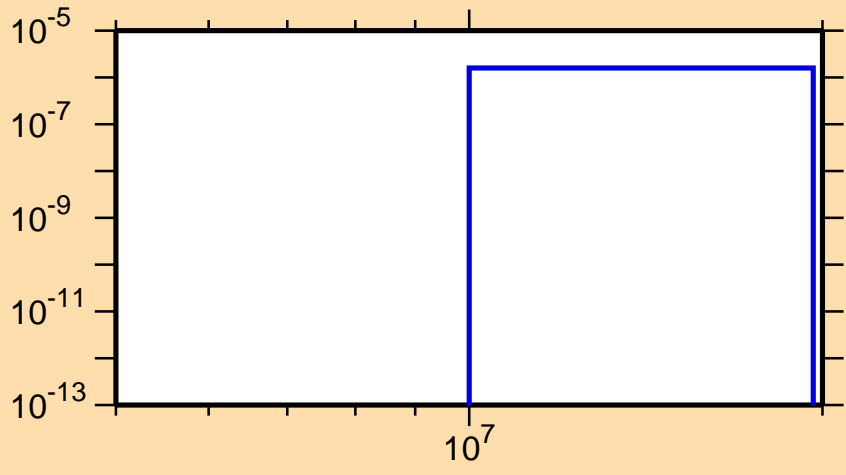
\sigma vs. E for ^{83}\text{Nb}(\text{mt } 45)
