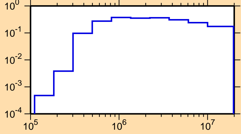
\sigma vs. E for ^{83}\text{Nb}(n,\text{inel.})
