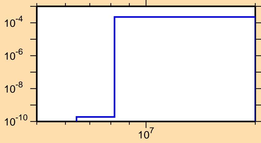
\sigma vs. E for ^{83}\text{Nb}(n,\alpha)
