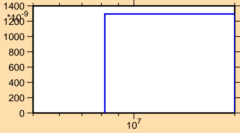
\sigma vs. E for ^{83}\text{Nb} (mt 45)
