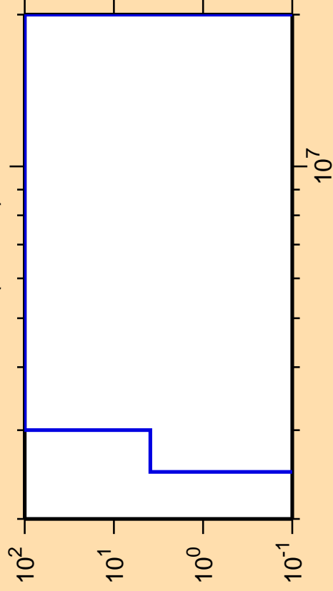
\Delta\sigma/\sigma vs. E for ^{83}\text{Nb}(n,\text{He3})
