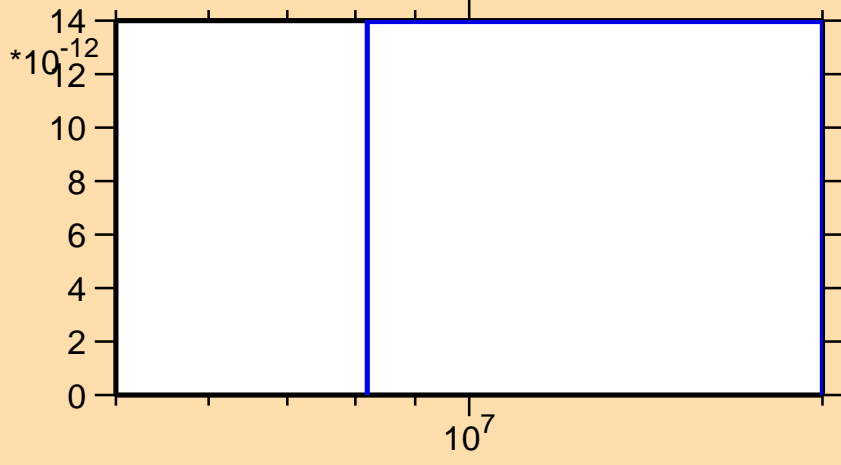
\sigma vs. E for ^{83}\text{Nb} (mt 34)
