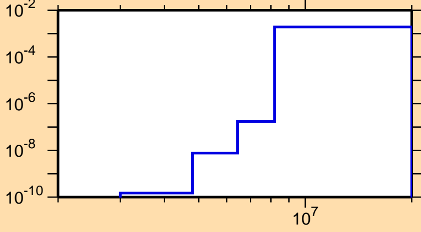
\sigma vs. E for ^{83}\text{Nb}(n,\text{He3})
