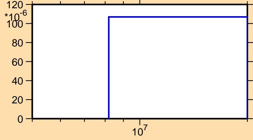
\sigma vs. E for ^{83}\text{Nb}(n,t)
