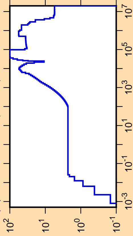
\Delta\mu/\mu vs. E for ^{84}\text{Nb}(\text{mt251})
