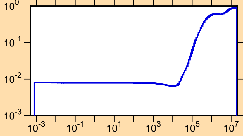
\mu vs. E for ^{84}\text{Nb}(\text{mt251})
