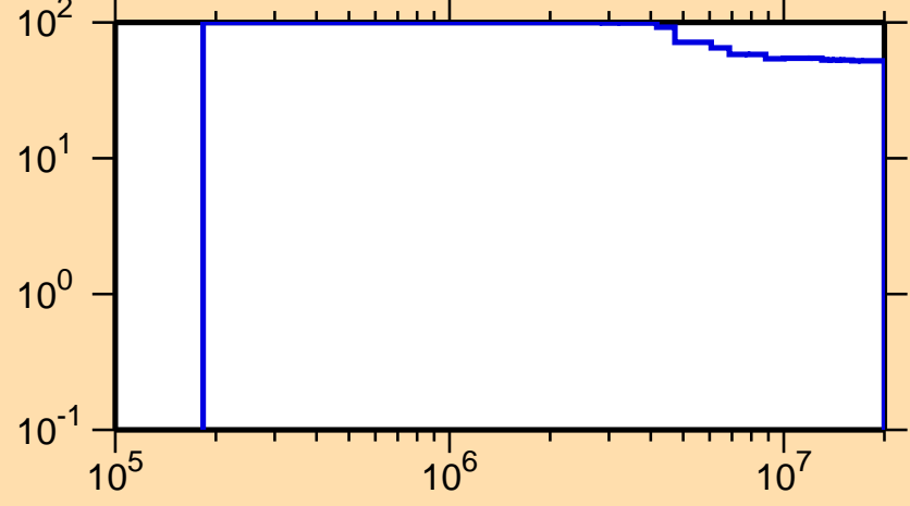
\Delta\sigma/\sigma vs. E for ^{84}\text{Nb}(n,n\text{cont.})
