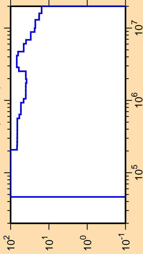
\Delta\sigma/\sigma vs. E for ^{84}\text{Nb}(n,\text{inel.})
