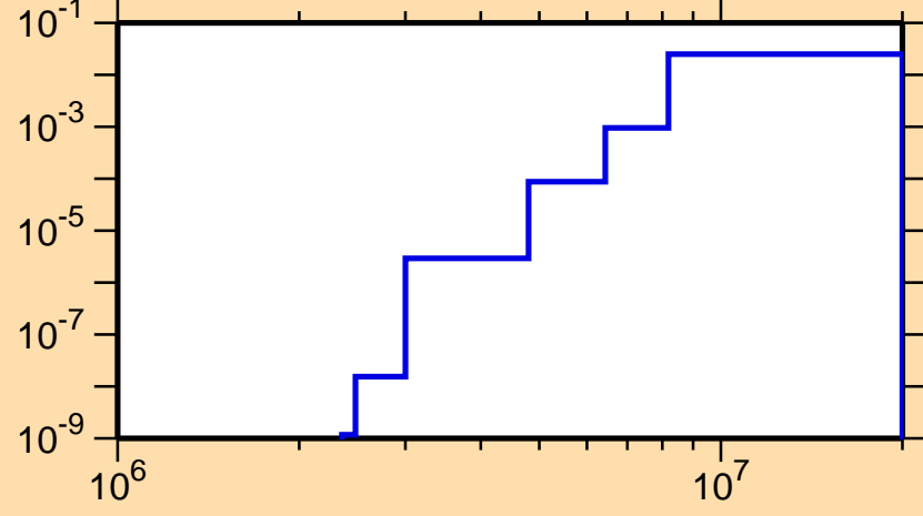
\sigma vs. E for ^{84}\text{Nb}(n,d)
