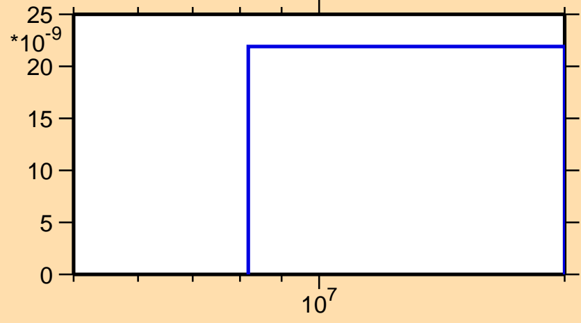
\sigma vs. E for ^{84}\text{Nb}(\text{mt117})
