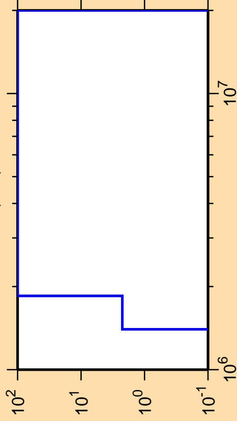
\Delta\sigma/\sigma vs. E for ^{84}\text{Nb}(n,d)
