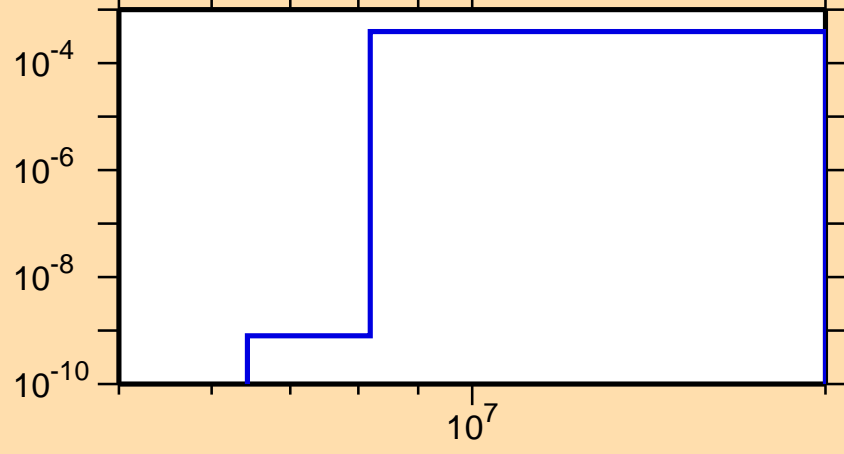
\sigma vs. E for ^{84}\text{Nb}(n,t)
