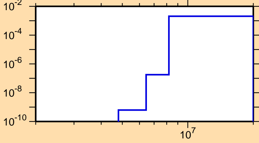
\sigma vs. E for ^{84}\text{Nb}(n,\text{He}3)
