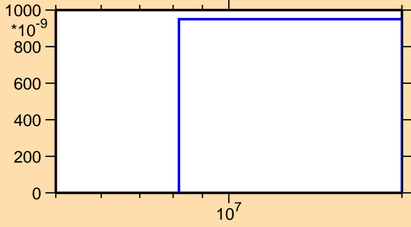
\sigma vs. E for ^{84}\text{Nb}(\text{mt } 45)
