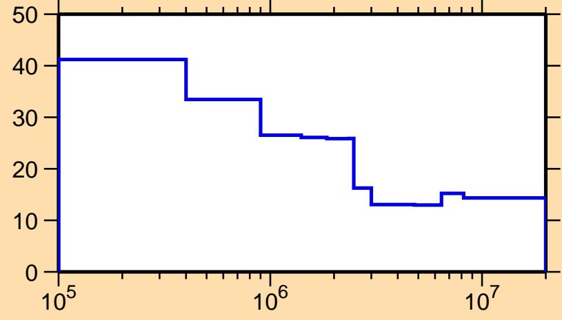
\Delta\sigma/\sigma vs. E for ^{84}\text{Nb}(n,n\text{nonel.})
