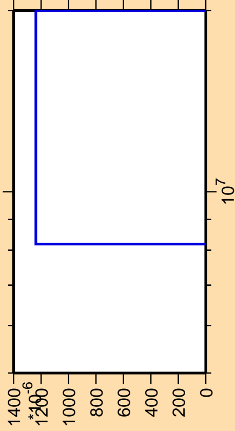
\Delta\sigma/\sigma vs. E for ^{84}\text{Nb}(n,2n\alpha)
