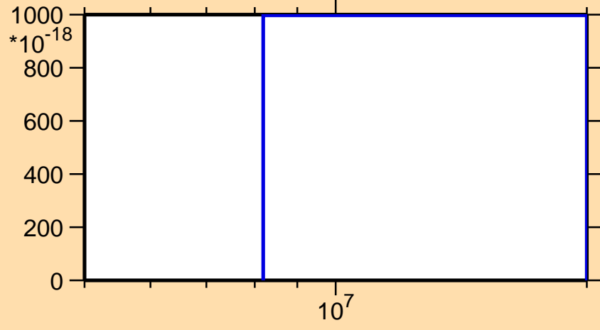
\sigma vs. E for ^{84}\text{Nb}(n,2n\alpha)
