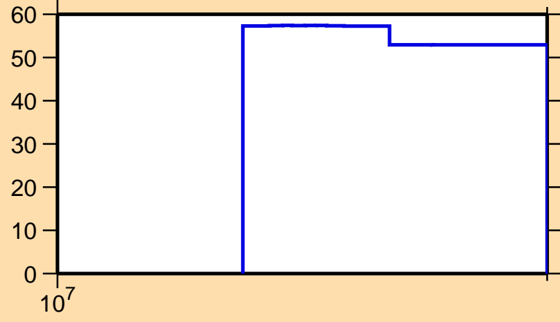
\Delta\sigma/\sigma vs. E for ^{85}\text{Nb}(n,\text{inel.})
