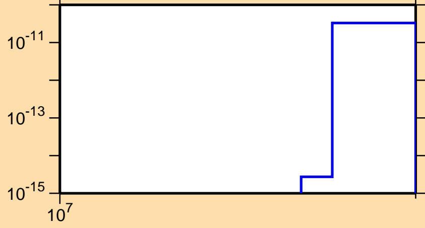
\sigma vs. E for ^{85}\text{Nb} (mt 34)
