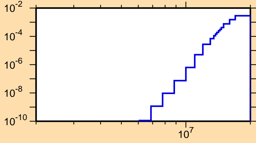
\sigma vs. E for ^{85}\text{Nb}(n,\text{He}3)
