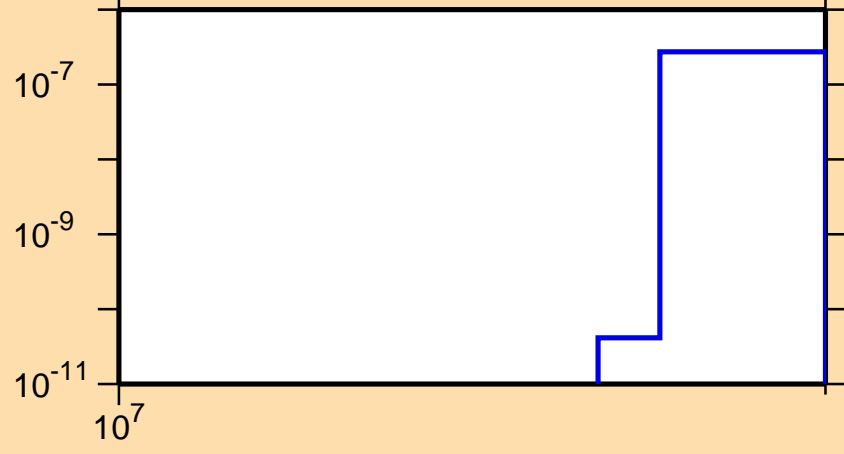
\sigma vs. E for ^{85}\text{Nb}(n,\text{pt})
