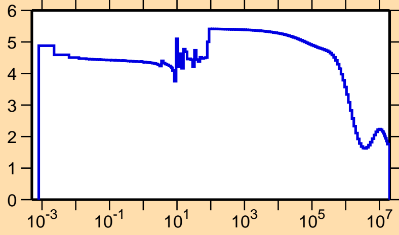
\sigma vs. E for ^{85}\text{Nb}(n,\text{el.})
