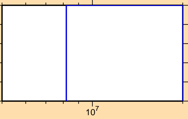
\sigma vs. E for ^{85}\text{Nb}(n,2n)
