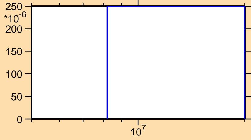
\sigma vs. E for ^{85}\text{Nb}(n,2n)
