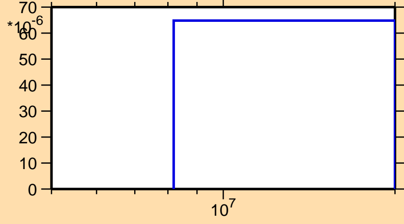
\sigma vs. E for ^{85}\text{Nb}(n,t)
