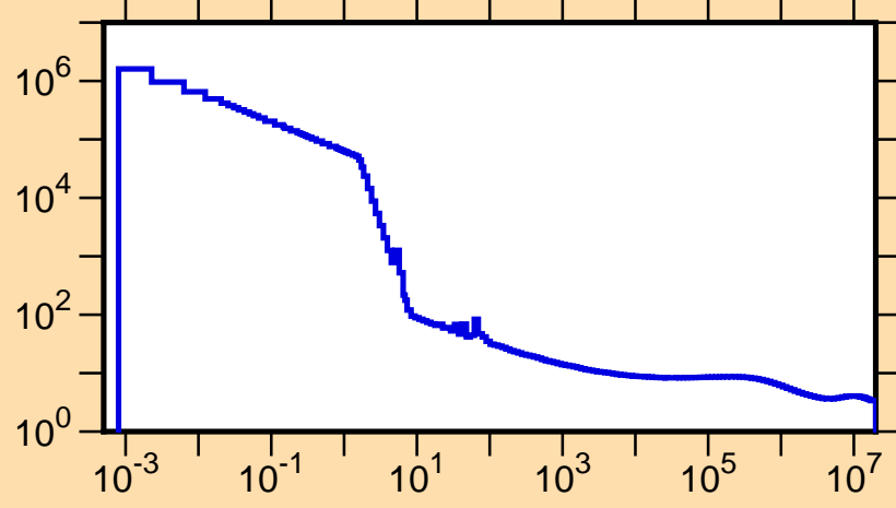
\sigma vs. E for ^{86}\text{Nb}(n,\text{tot.})
