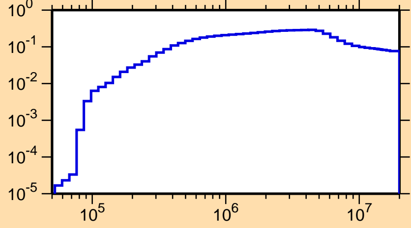
\sigma vs. E for ^{86}\text{Nb}(n,\text{inel.})
