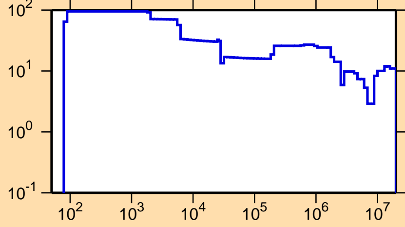
\Delta\sigma/\sigma vs. E for ^{86}\text{Nb}(n,\text{tot.})
