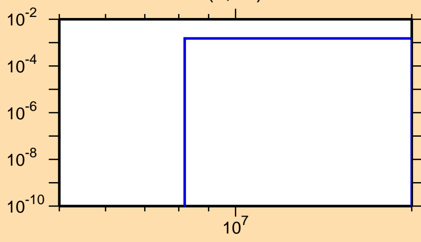
\sigma vs. E for ^{86}\text{Nb}(n,\alpha)
