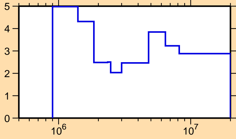
\Delta\sigma/\sigma vs. E for ^{87}\text{Nb}(n,\text{nonel.})
