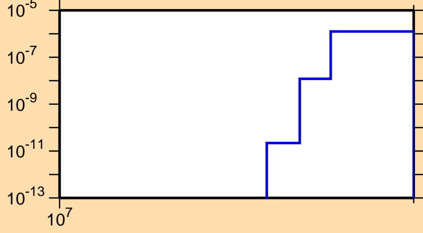
\sigma vs. E for ^{87}\text{Nb}(n,\text{nd})
