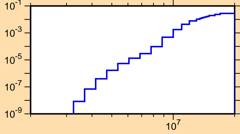
\sigma vs. E for ^{87}\text{Nb}(n,d)
