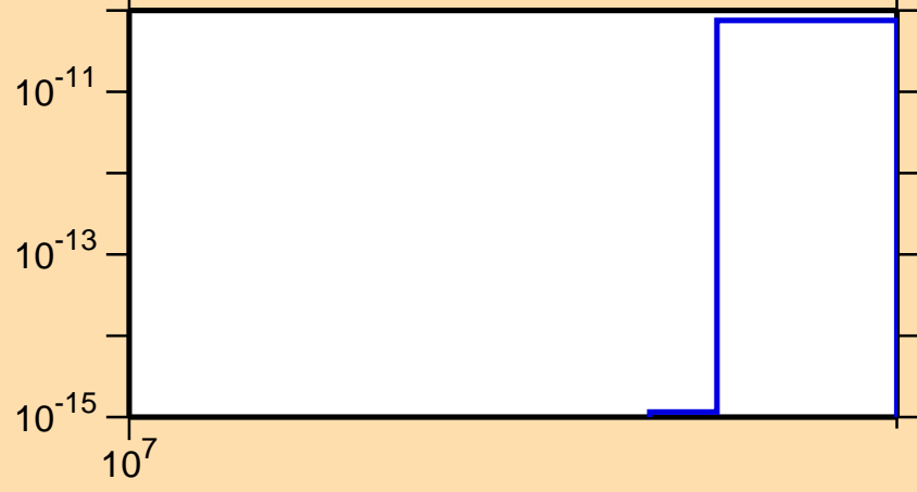
\sigma vs. E for ^{88}\text{Nb} (mt 34)
