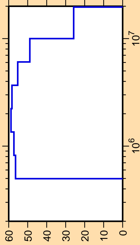
\Delta\sigma/\sigma vs. E for ^{88}\text{Nb}(n,n_2)
