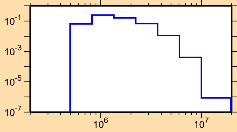
\sigma vs. E for ^{88}\text{Nb}(n,n_2)
