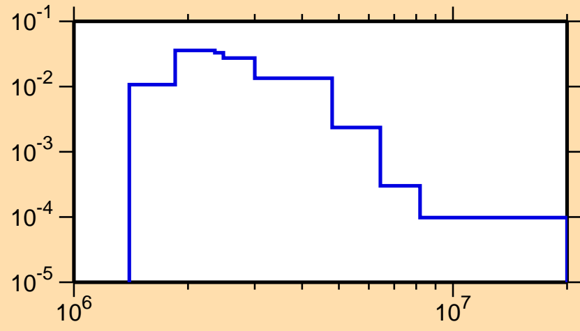
\sigma vs. E for ^{88}\text{Nb}(n,n_4)
