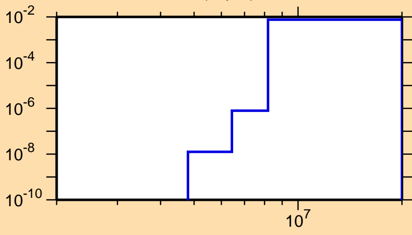
\sigma vs. E for ^{88}\text{Nb}(n,p\alpha)
