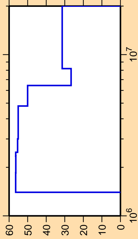
\Delta\sigma/\sigma vs. E for ^{88}\text{Nb}(n,n_4)
