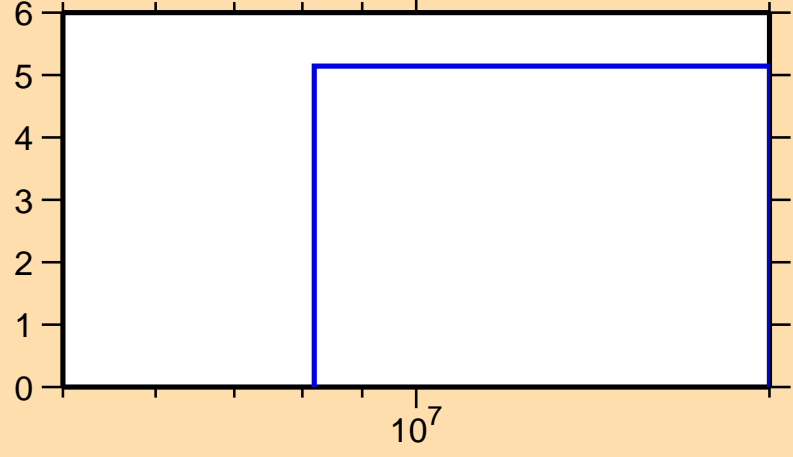
\Delta\sigma/\sigma vs. E for ^{88}\text{Nb}(n,\text{tot.})
