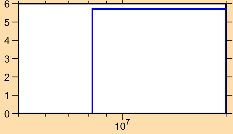
\Delta\sigma/\sigma vs. E for ^{88}\text{Nb}(n,\text{el.})
