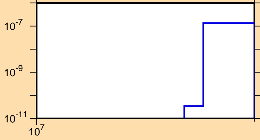
\sigma vs. E for ^{88}\text{Nb}(n,\text{pt})
