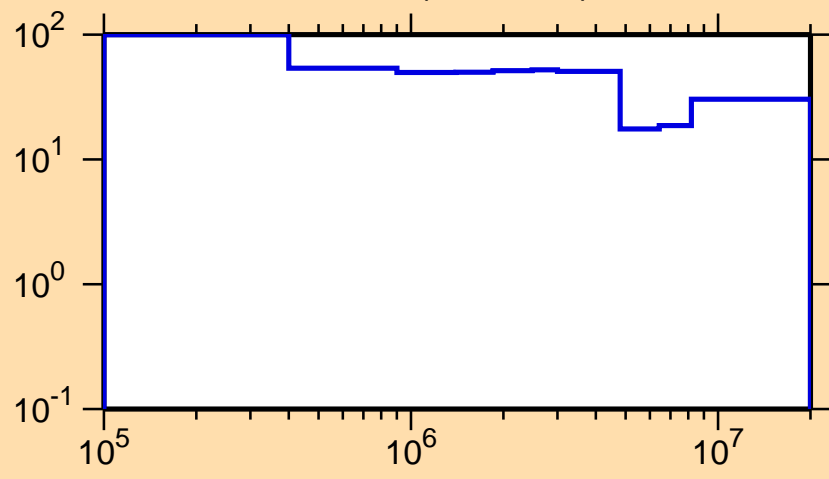
\Delta\sigma/\sigma vs. E for ^{88}\text{Nb}(n,n\text{cont.})
