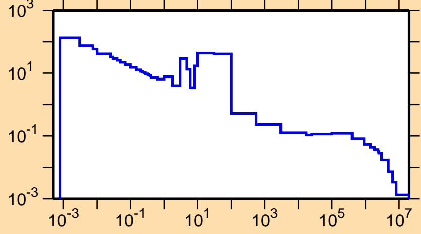
\sigma vs. E for ^{88}\text{Nb}(n,\gamma)
