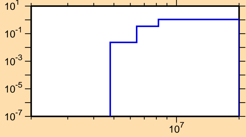
\sigma vs. E for ^{88}\text{Nb}(n,np)
