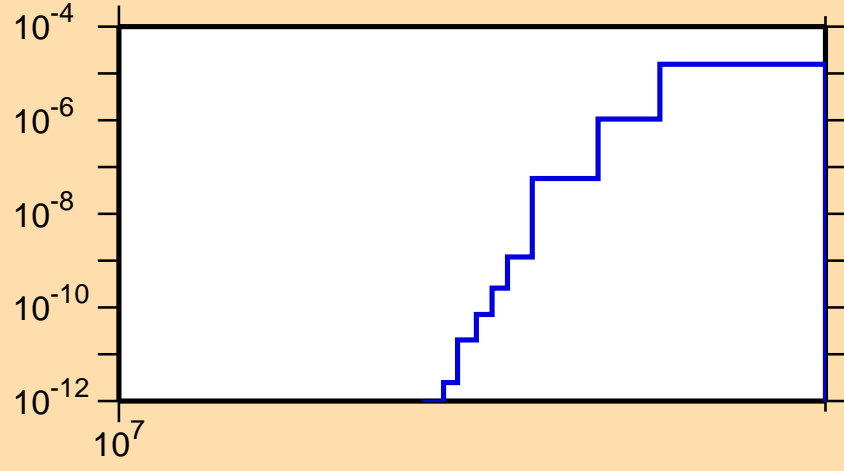
\sigma vs. E for ^{89}\text{Nb}(n,pd)
