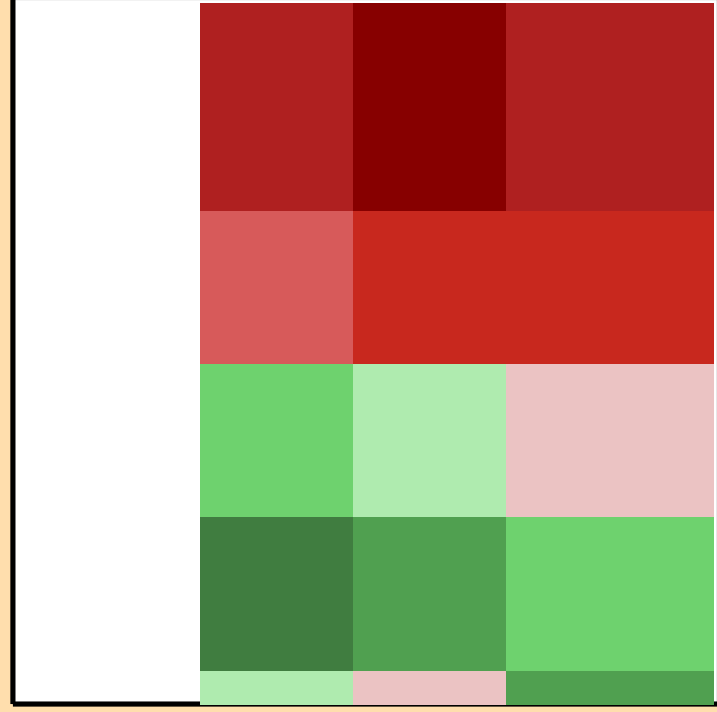
\Delta\sigma/\sigma vs. E for ^{89}\text{Nb}(n,ncont.)
