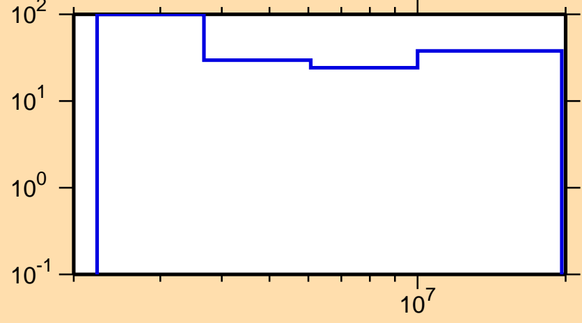
\Delta\sigma/\sigma vs. E for ^{89}\text{Nb}(n,ncont.)
