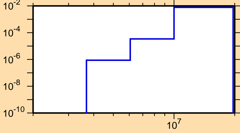
\sigma vs. E for ^{89}\text{Nb}(n,d)
