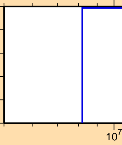
\sigma vs. E for ^{89}\text{Nb}(n,2np)
