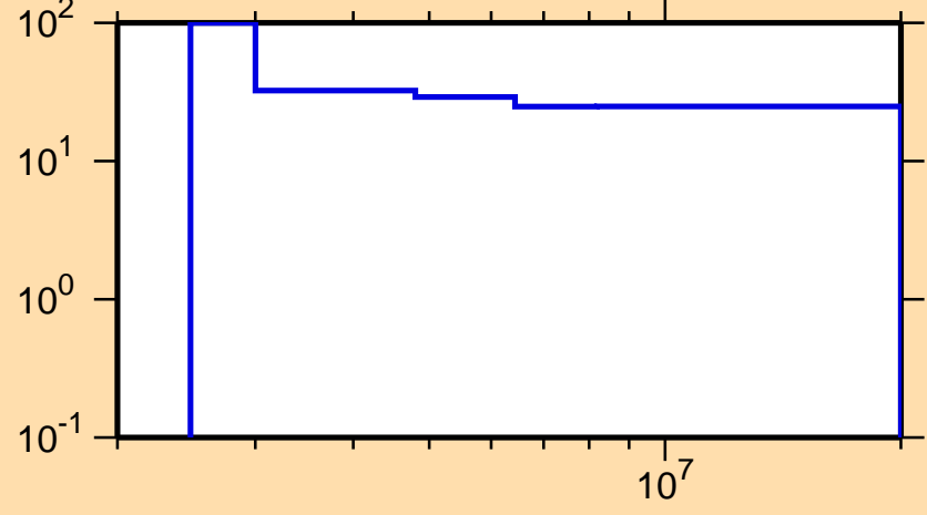
\Delta\sigma/\sigma vs. E for ^{89}\text{Nb}(n,n\text{cont.})
