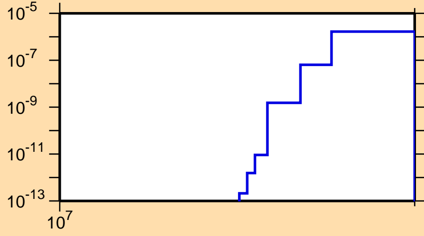
\sigma vs. E for ^{90}\text{Nb}(n,pd)
