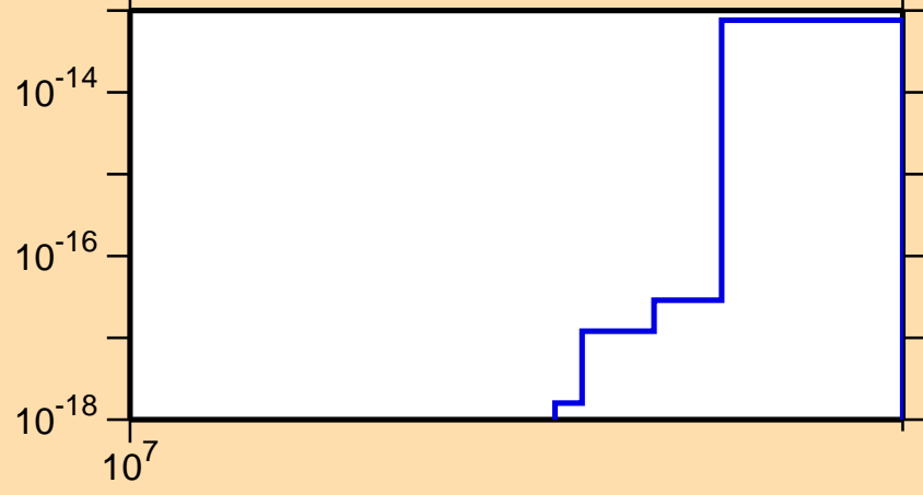
\sigma vs. E for ^{90}\text{Nb} (mt 34)
