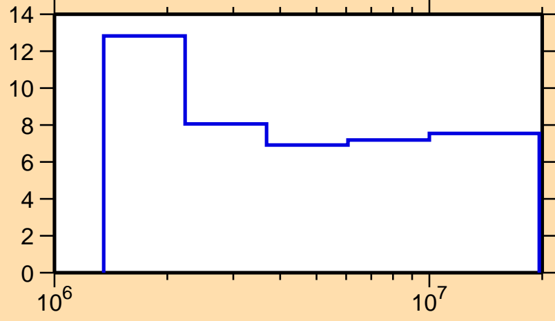
\Delta\sigma/\sigma vs. E for ^{90}\text{Nb}(n,n\text{nonel.})
