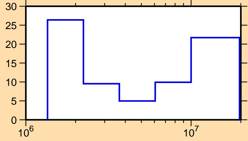
\Delta\sigma/\sigma vs. E for ^{90}\text{Nb}(n,ncont.)
