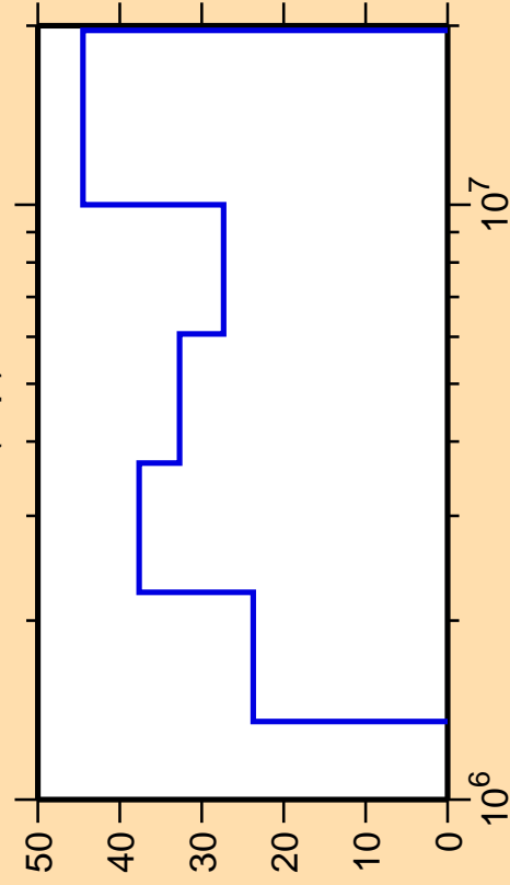
\Delta\sigma/\sigma vs. E for ^{90}\text{Nb}(n,p)
