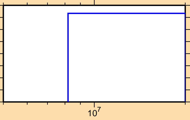
\sigma vs. E for ^{90}\text{Nb}(n,\text{pt})
