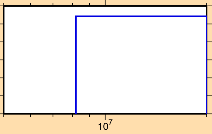
\sigma vs. E for ^{90}\text{Nb}(n,\text{nd})
