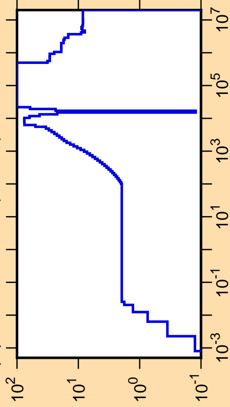
\Delta\mu/\mu vs. E for ^{91}\text{Nb}(\text{mt251})
