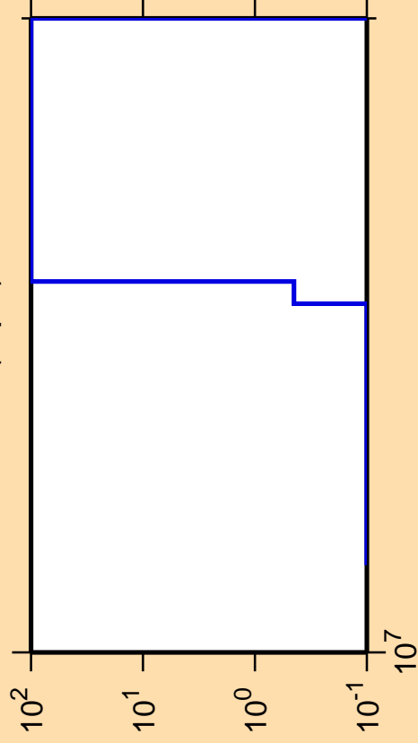
\Delta\sigma/\sigma vs. E for ^{91}\text{Nb}(n,pd)
