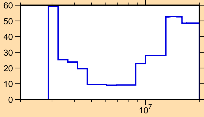
\Delta\sigma/\sigma vs. E for ^{91}\text{Nb}(n,ncont.)
