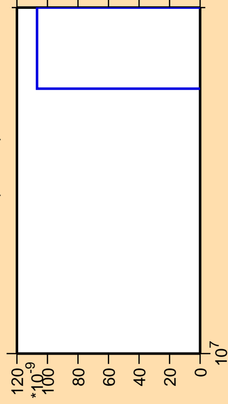
\Delta\sigma/\sigma vs. E for ^{91}\text{Nb}(n,2n\alpha)
