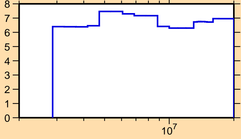
\Delta\sigma/\sigma vs. E for ^{91}\text{Nb}(n,\text{nonel.})
