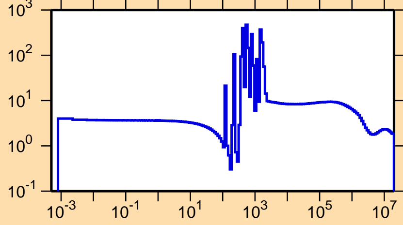
\sigma vs. E for ^{91}\text{Nb}(n,\text{el.})
