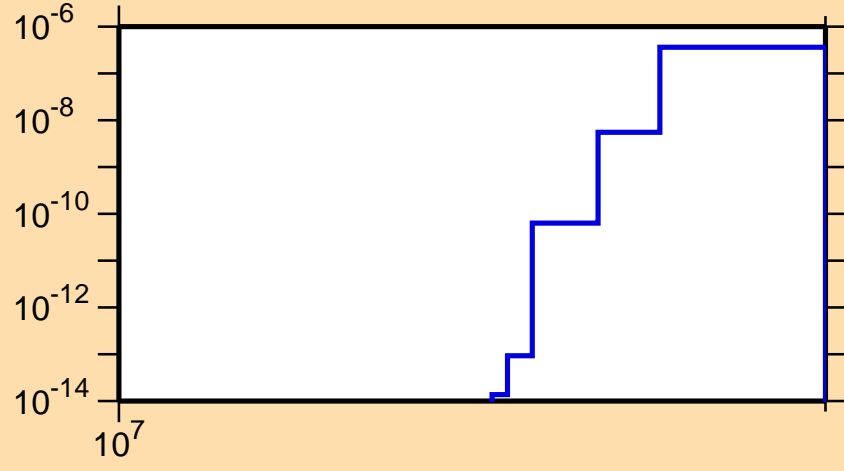
\sigma vs. E for ^{91}\text{Nb}(n,pd)
