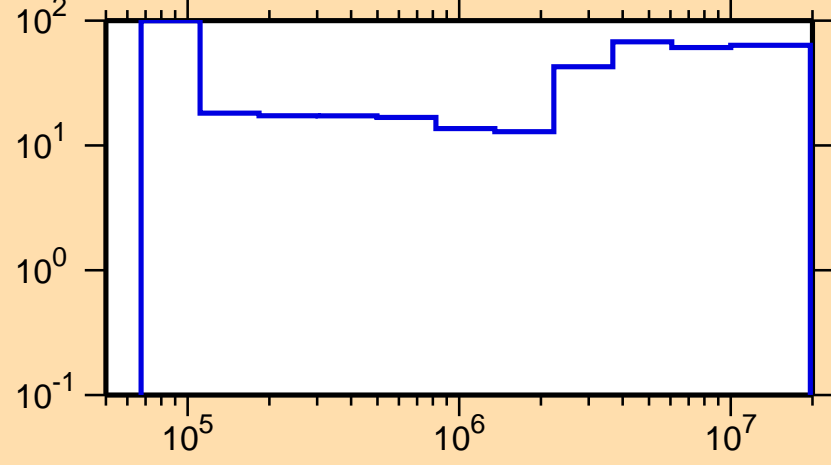
\Delta\sigma/\sigma vs. E for ^{91}\text{Nb}(n,n_1)
