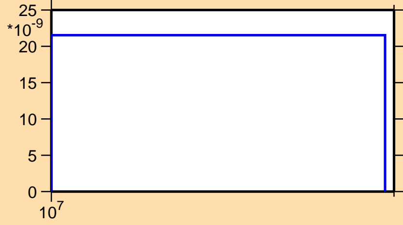
\sigma vs. E for ^{91}\text{Nb}(n,2np)
