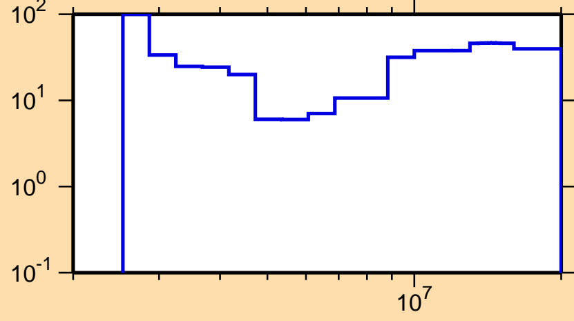
\Delta\sigma/\sigma vs. E for ^{91}\text{Nb}(n,ncont.)
