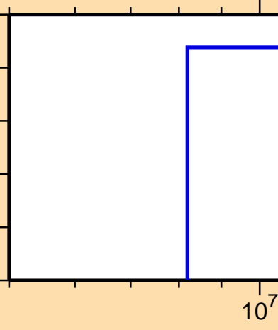
\sigma vs. E for ^{91}\text{Nb}(n,t)
