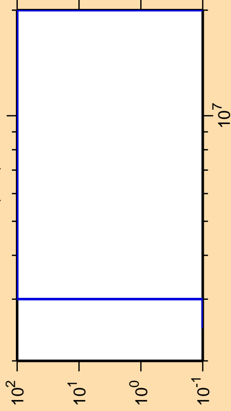
\Delta\sigma/\sigma vs. E for ^{91}\text{Nb}(n,d)
