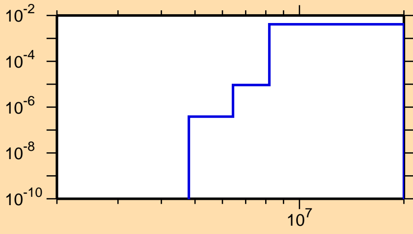
\sigma vs. E for ^{91}\text{Nb}(n,d)
