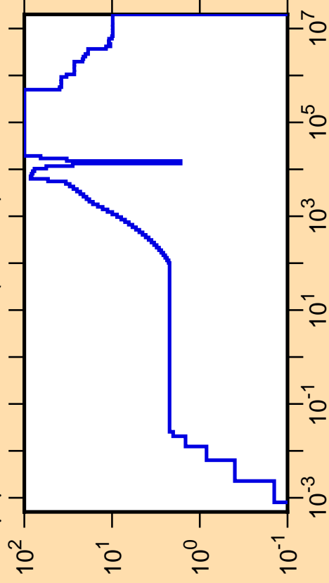
\Delta\mu/\mu vs. E for ^{92}\text{Nb}(\text{mt251})
