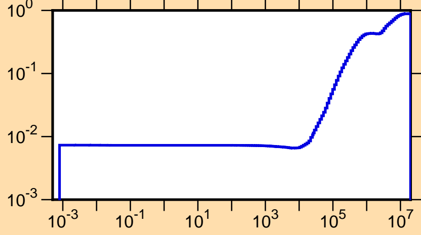
\mu vs. E for ^{92}\text{Nb}(\text{mt251})
