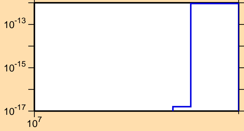
\sigma vs. E for ^{92}\text{Nb} (mt 45)
