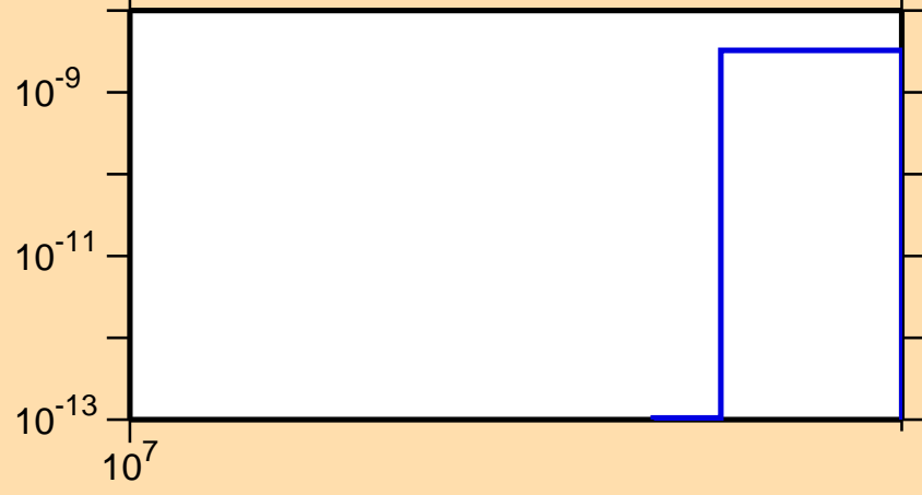
\sigma vs. E for ^{92}\text{Nb}(n,\text{pt})
