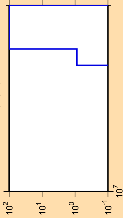
\Delta\sigma/\sigma vs. E for ^{92}\text{Nb}(n,pd)
