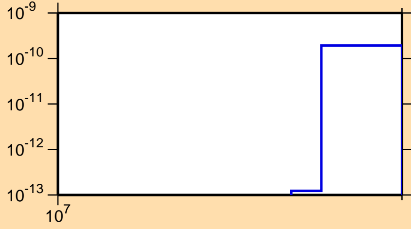
\sigma vs. E for ^{92}\text{Nb}(n,pd)
