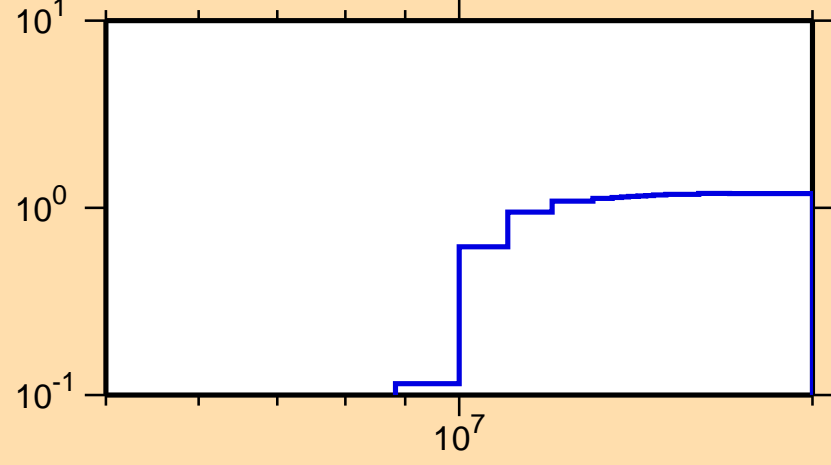
\sigma vs. E for ^{93}\text{Nb}(n,2n)
