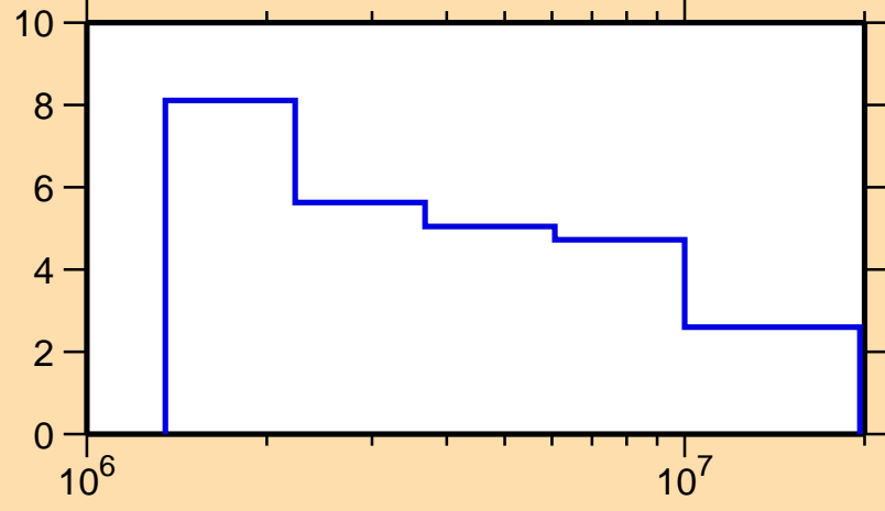
\Delta\sigma/\sigma vs. E for ^{93}\text{Nb}(n,n\text{nonel.})
