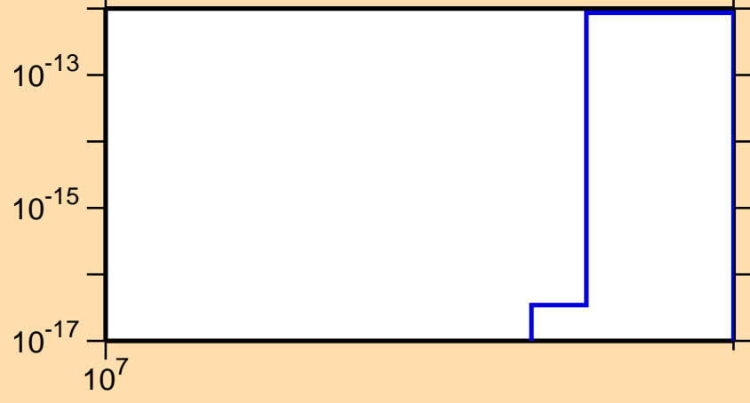
\sigma vs. E for ^{93}\text{Nb}(n,\text{pd})
