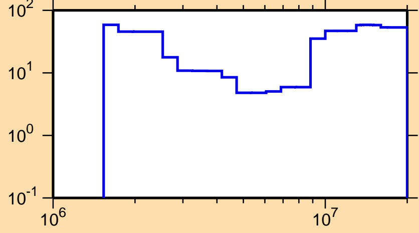
\Delta\sigma/\sigma vs. E for ^{93}\text{Nb}(n,n\text{cont.})
