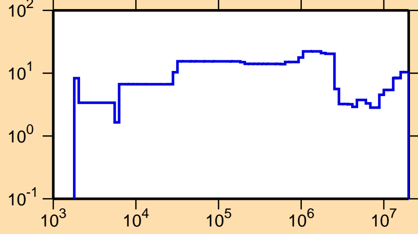
\Delta\sigma/\sigma vs. E for ^{93}\text{Nb}(n,\text{el.})
