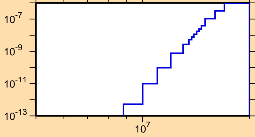
\sigma vs. E for ^{93}\text{Nb}(n,p\alpha)
