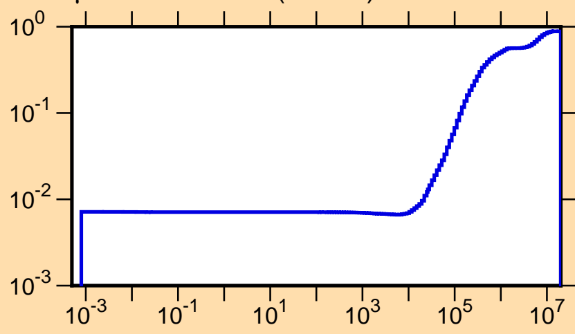
\mu vs. E for ^{94}\text{Nb}(\text{mt251})
